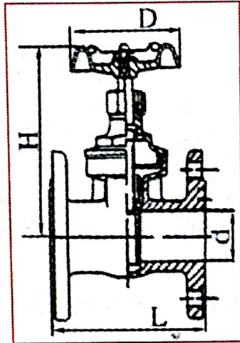
黄铜法兰闸阀 Brass Gate Valve (flanged) Unit: mm
