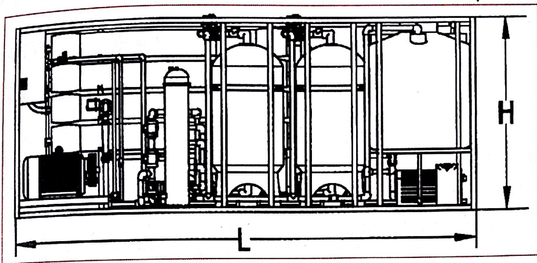
反渗透海水淡化装置 Reverse Osmosis Fresh Water Generator
