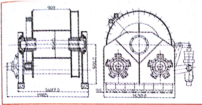
YB120液压绞车 Hydraulic Winch
