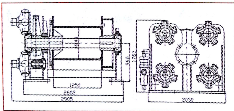
YQJ400 液压绞车 Hydraulic Winch
