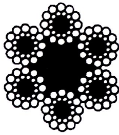
6×24S+7FC
