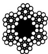
6 × 19S+FC
