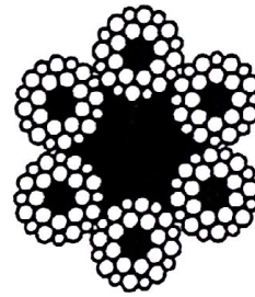
6×24W+7FC
